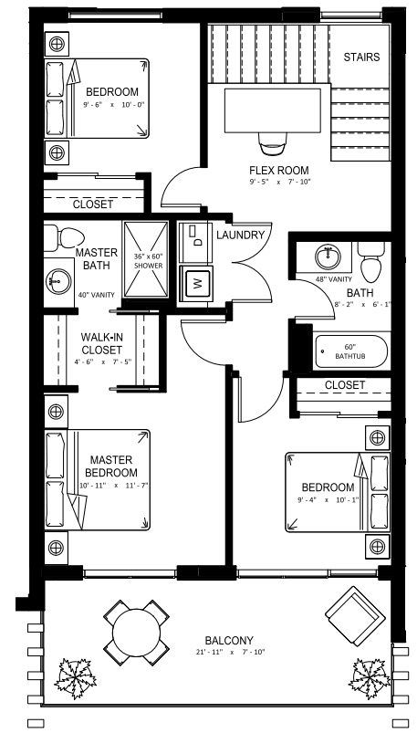
Second Floor - 753 Sq.Ft.
